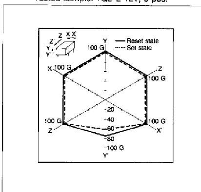
13.-(3) Influence of adjacent mounting
